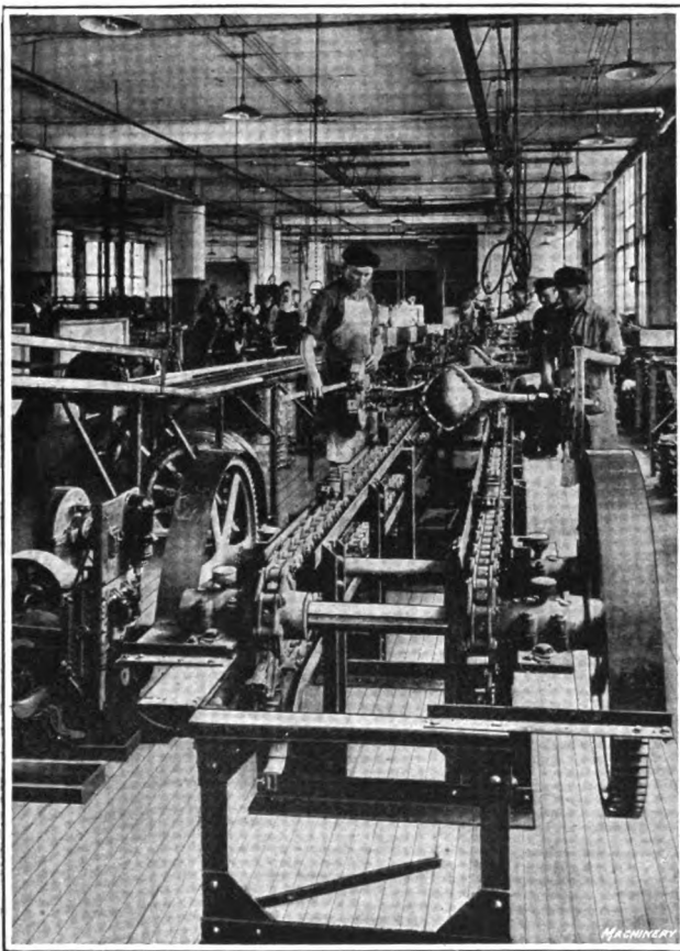
Fig. 26—The Palmer-Bee Co., of Detroit, Mich., makes a specialty of designing and installing time and labor-saving equipments for handling material in course of manufacture. This illustration shows an outfit installed by this company for assembling automobile transmissions. Two strands of endless chain carry brackets which support the work at each end
